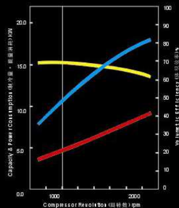
HCS-48 Performance Curve 性能曲线
