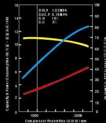
HCS-33 Performance Curve 性能曲线
